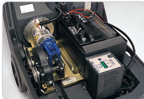
No tools required to access brooms and filter. Hood opens providing full maintenance accessibility to the cleanly engineered internal systems.
